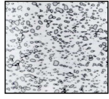
An alloy of aluminium with 4% copper (Duralumin) can be cooled to produce a fine dispersion of fine precipitates of hard CuAl2.
