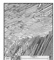
Steel is strengthened by Iron Carbide Precipitates.
